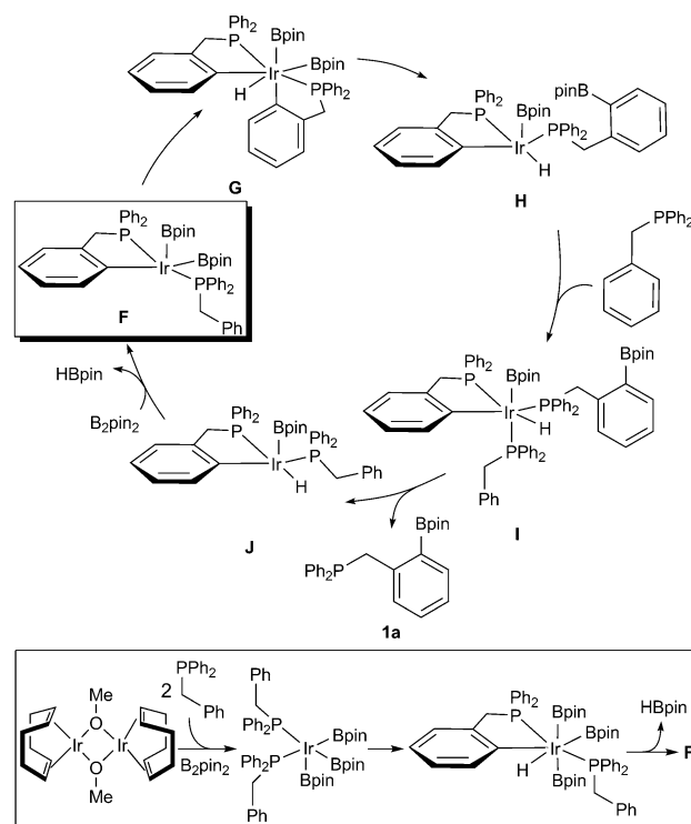
Scheme 5. Proposed catalytic cycle of C–H borylation.
